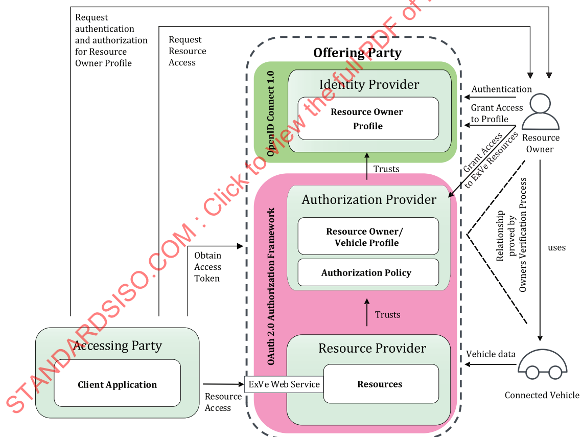
Figure 6 — Involved roles and associated entities
