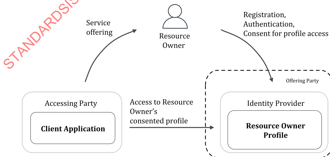
Figure 2 — Resource Owner Authentication and Access to Resource Owner's Profile
