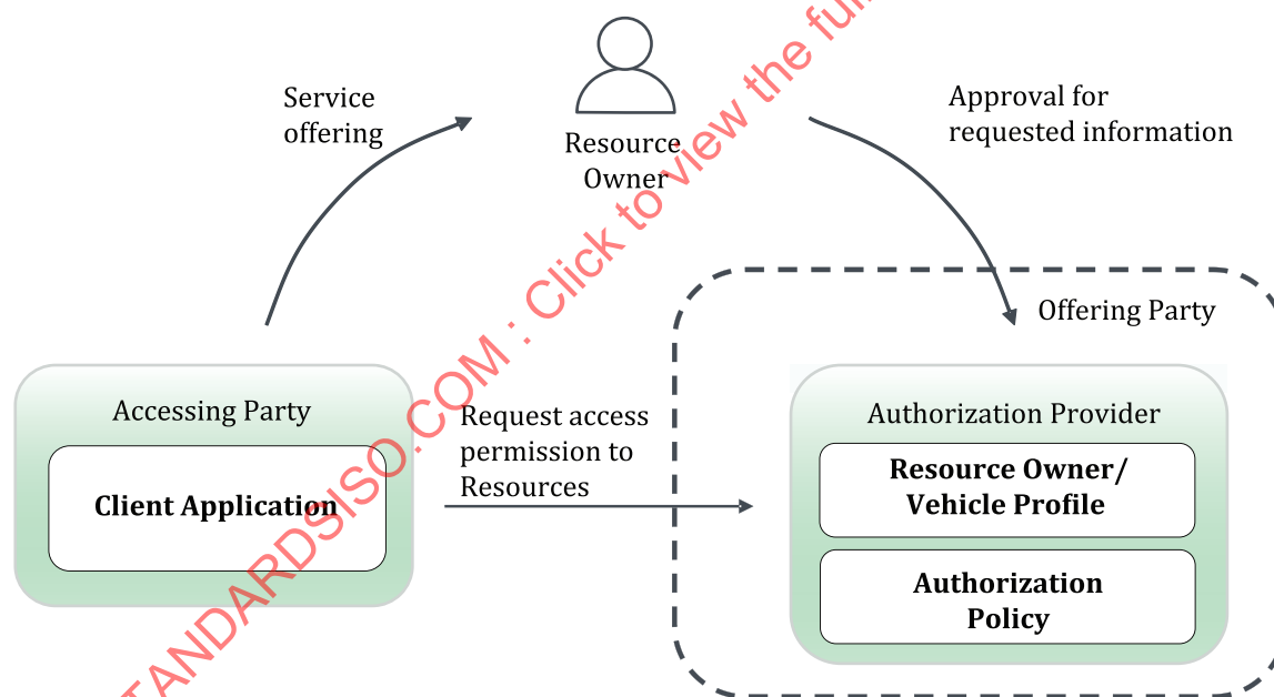
Figure 3 — Requesting Access to Resources
