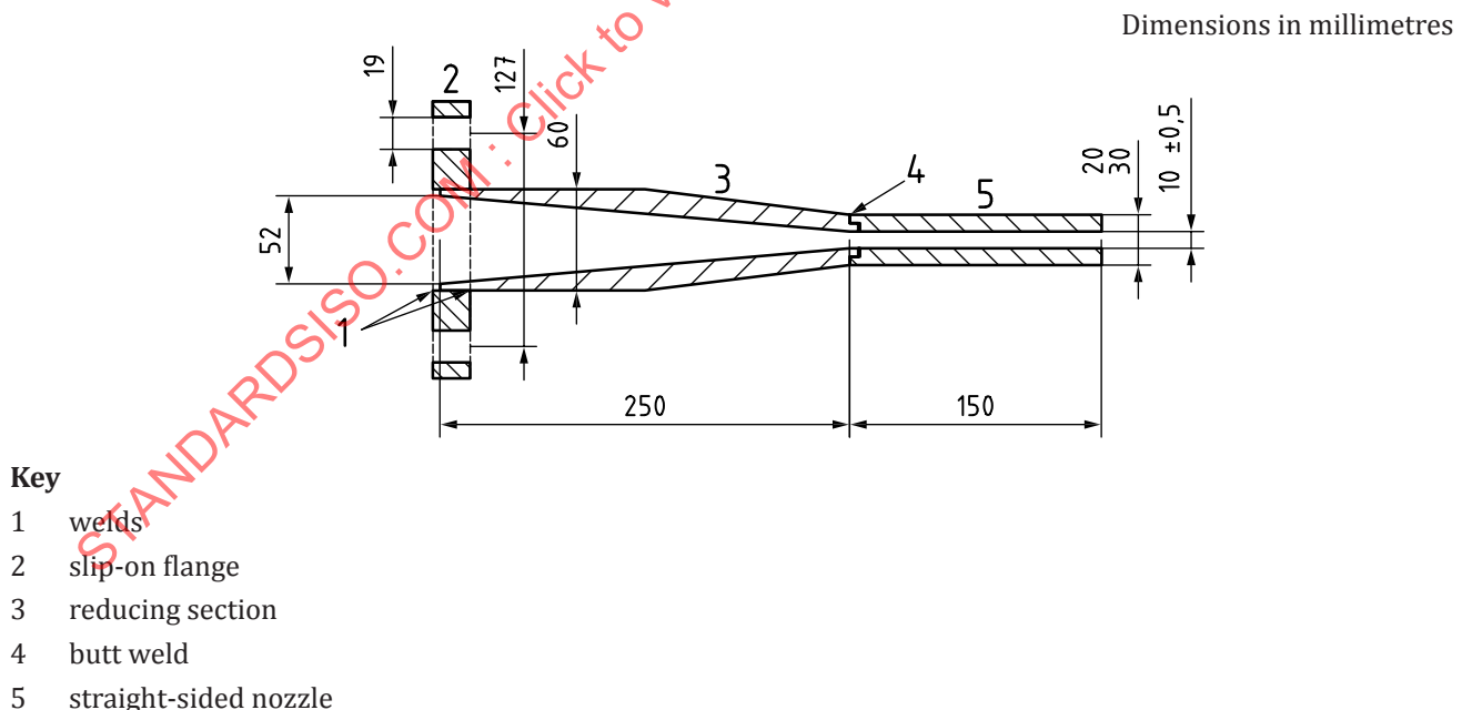
Figure 1 — Feed pipe and nozzle construction
