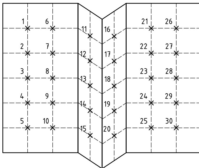
Figure 4 — Thickness measurement points for test specimen
