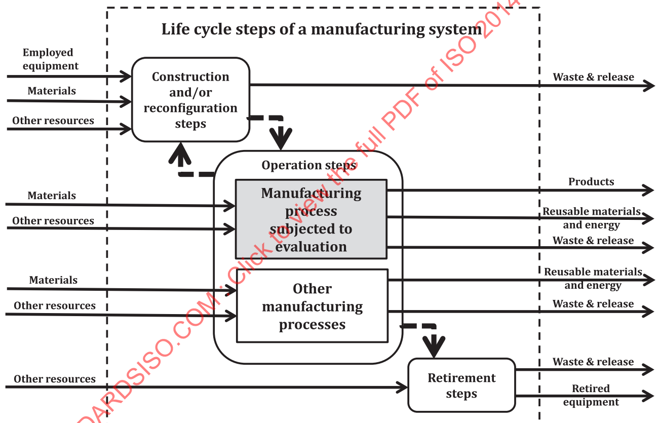
Figure 2 — Environmental influence resulting from the life cycle steps of a manufacturing system
