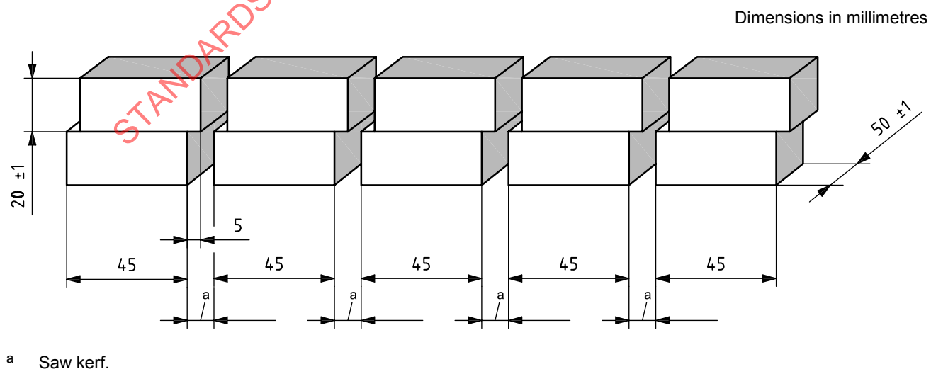
Figure 1 — Shear block assembly dimensions
