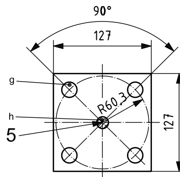
e) Spacer plate No. 2, 10 mm (stainless steel, one required)
