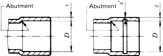
Fittings from pressings or castings
