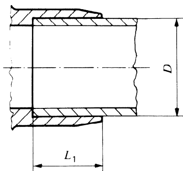
Figure 1 — Socket
