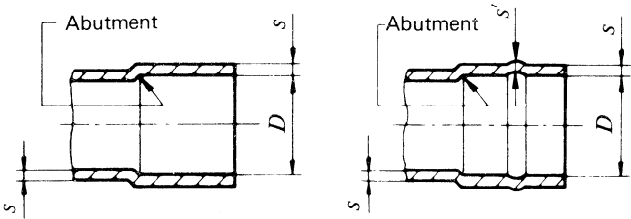
Fittings from drawn tube
