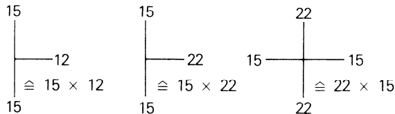
Figure 6 — Designation of tees and crosses equal on the run, reducing or increasing on the branch and symmetrically reducing on the branches
