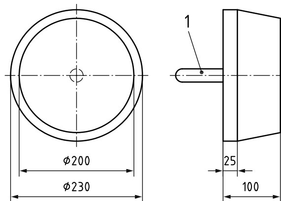
c) Probe D (large head)
