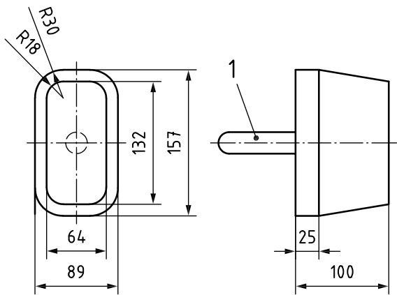
a) Probe E (small head)
