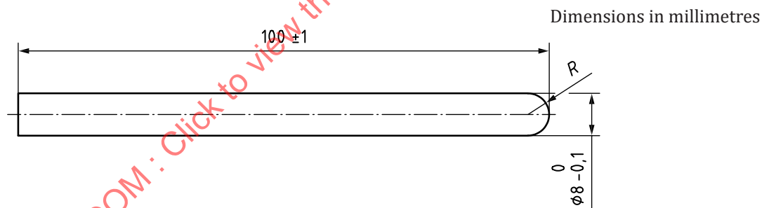
Figure 2 — 8 mm finger rod
