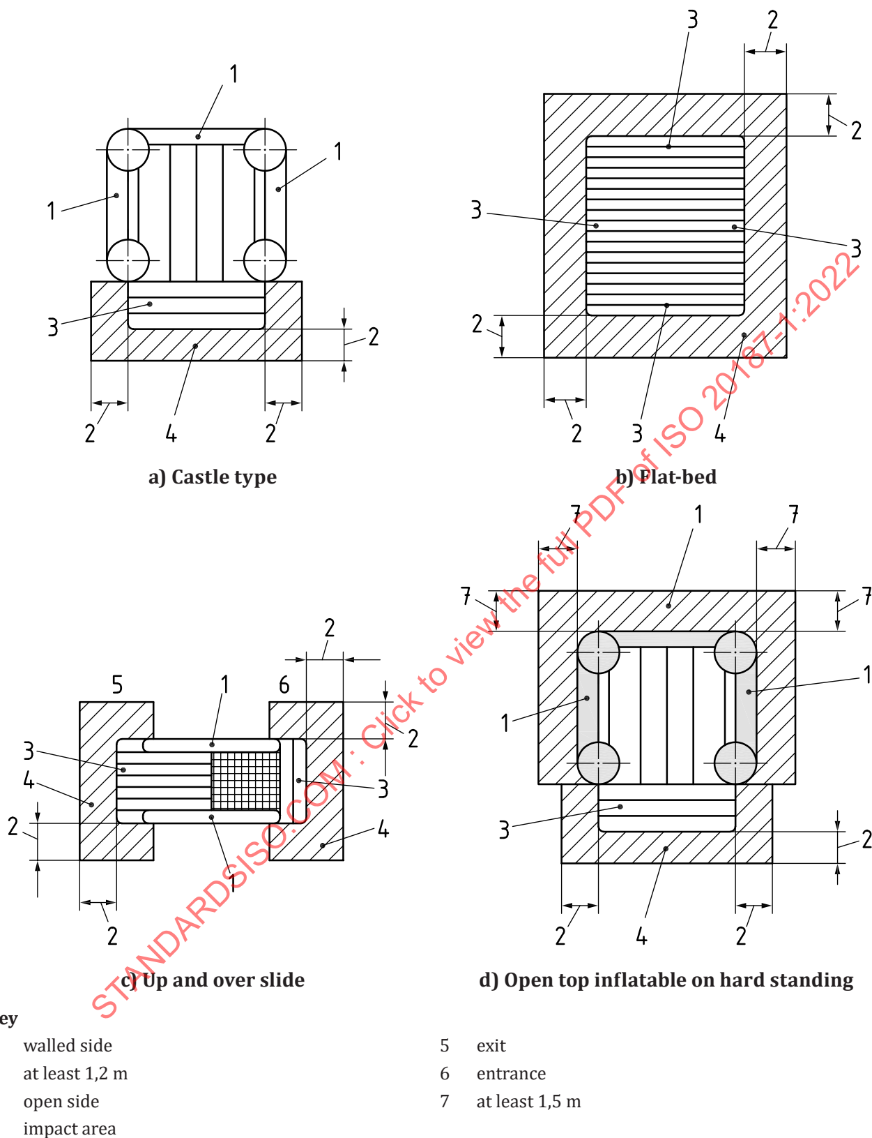
Figure 7 — Impact areas
