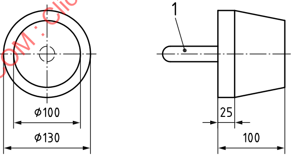
a) Probe E (small head)
