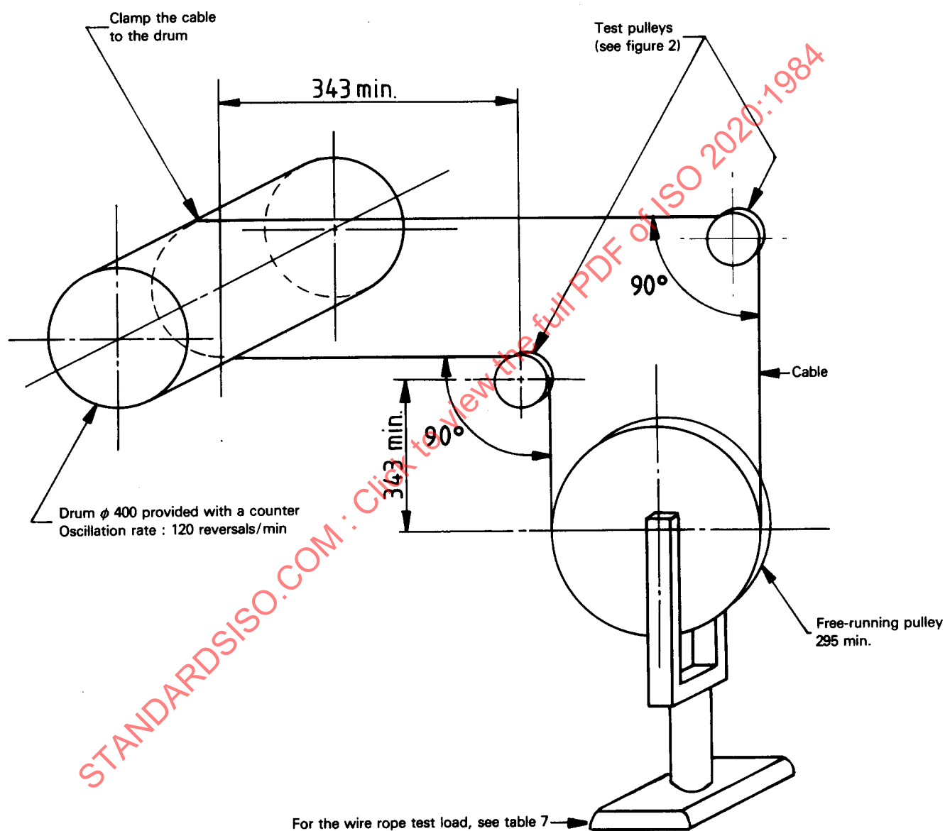
Figure 1 — Schematic diagram for endurance test — Equipment and test conditions
