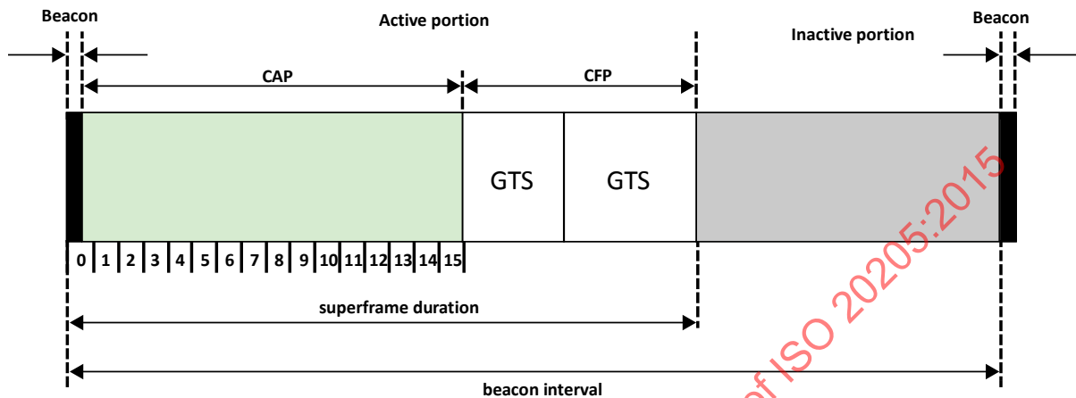
Figure 2-1: IEEE 802.15.4 Superframe
