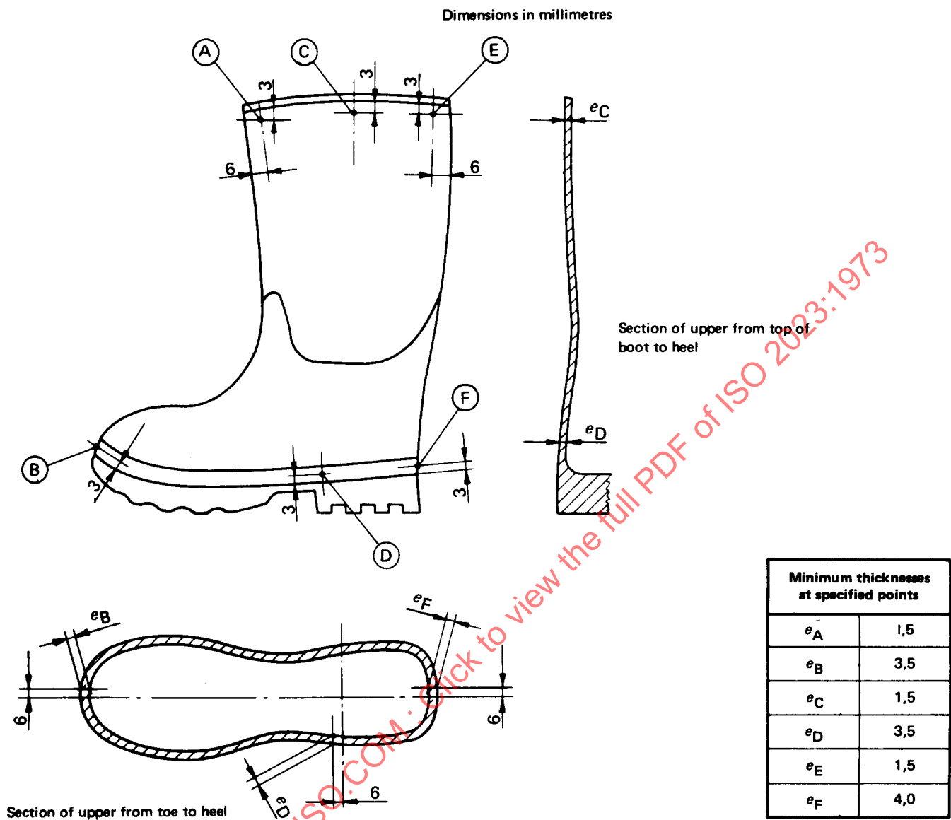
FIGURE 1 – Industrial rubber boot
