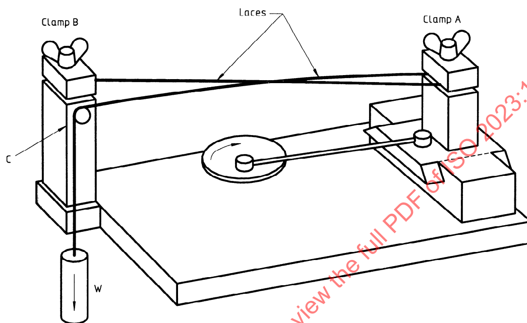
Figure B.1 — Lace-abrading machine
