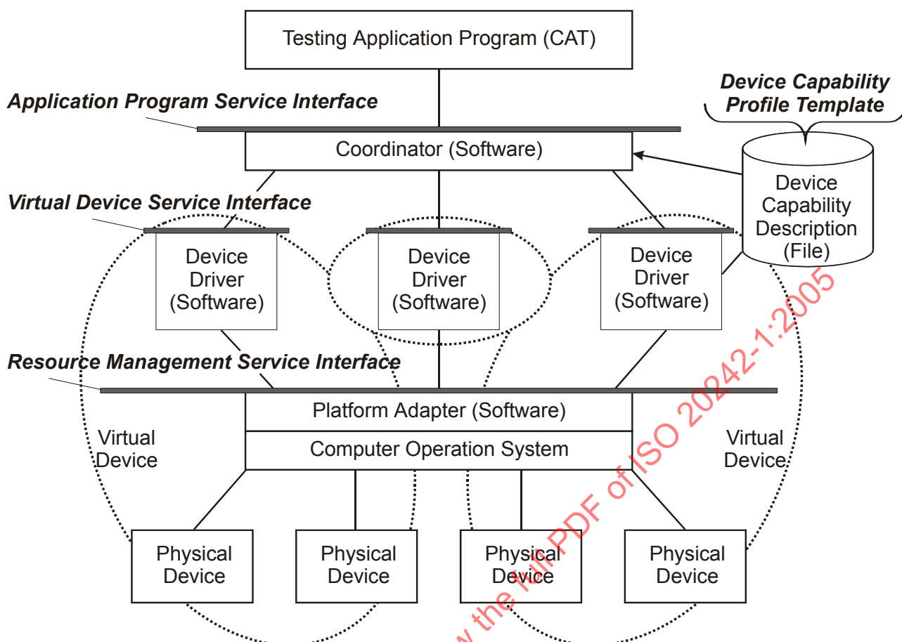
Figure 1 — Service interfaces defined in ISO 20242
