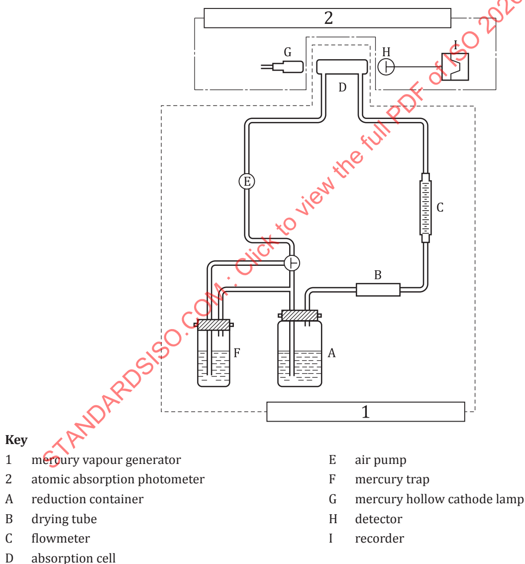
Figure 1 — Example of a closed circulating system for the measurement of mercury
