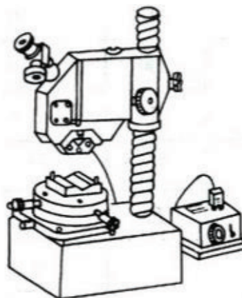
Figure A.2 — Example of a typical light-section microscope
