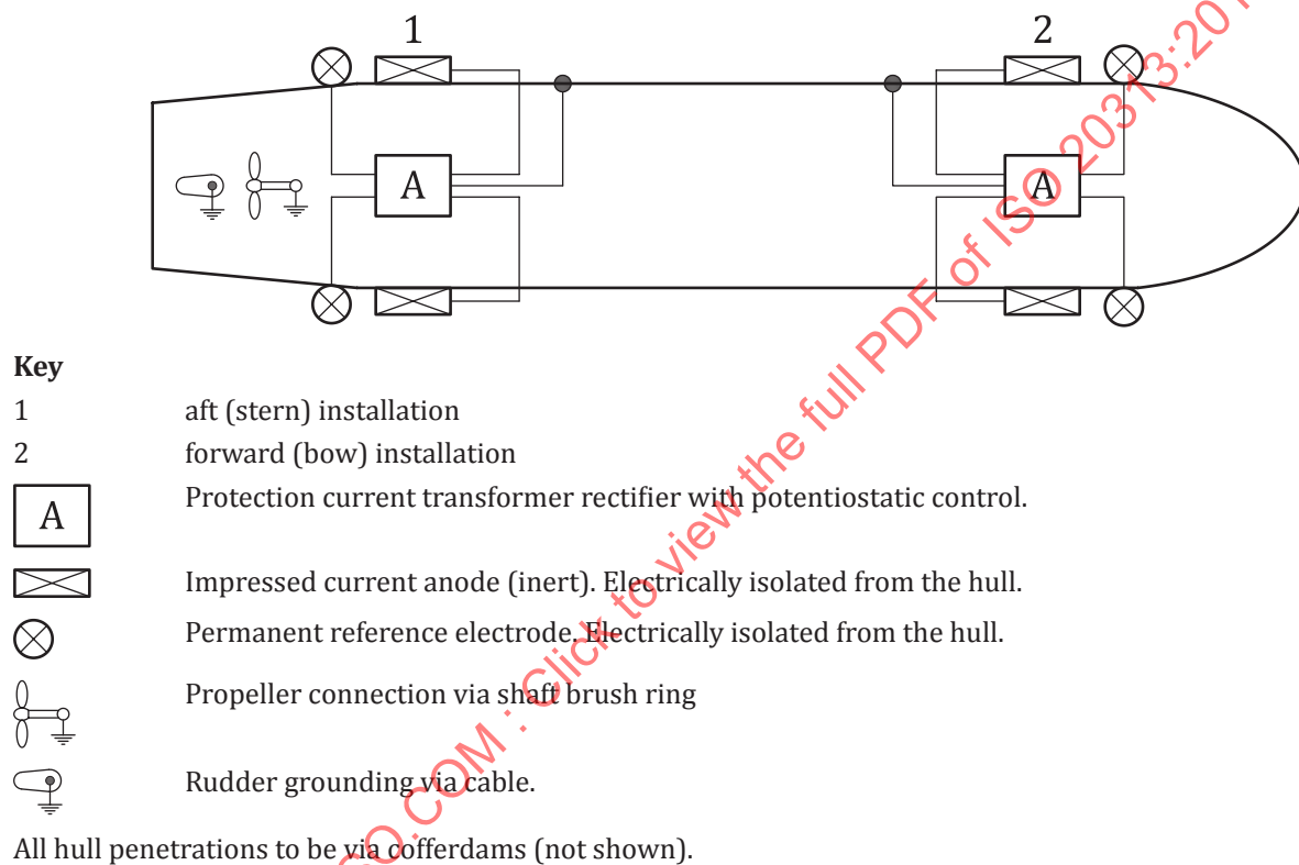
Figure A.1 — Typical schematic arrangement for an impressed current system for hulls of ships based on two cathodic protection zones
