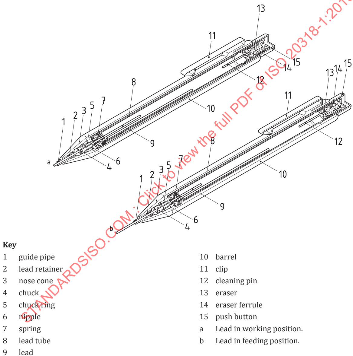
Figure 1 — Mechanical pencil of push-type F
