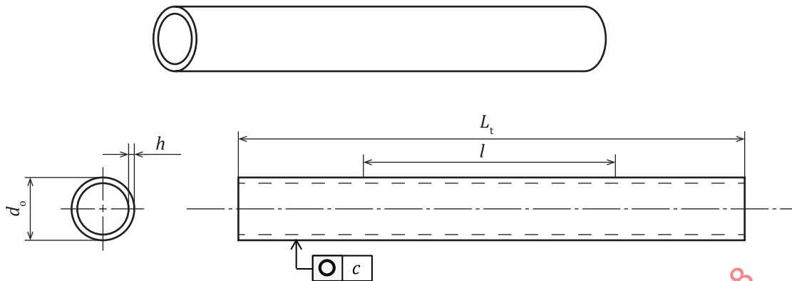
Figure 2 — “Generic” straight-sided tube test specimen
