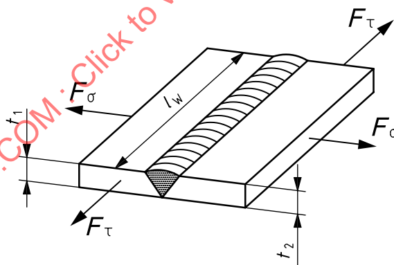
Figure C.1 — Butt weld
