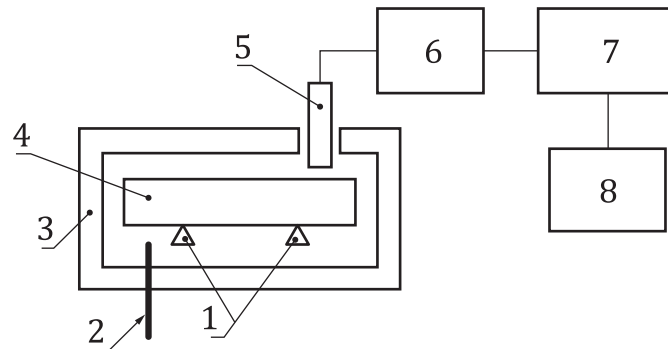
a) Impulse excitation testing method
