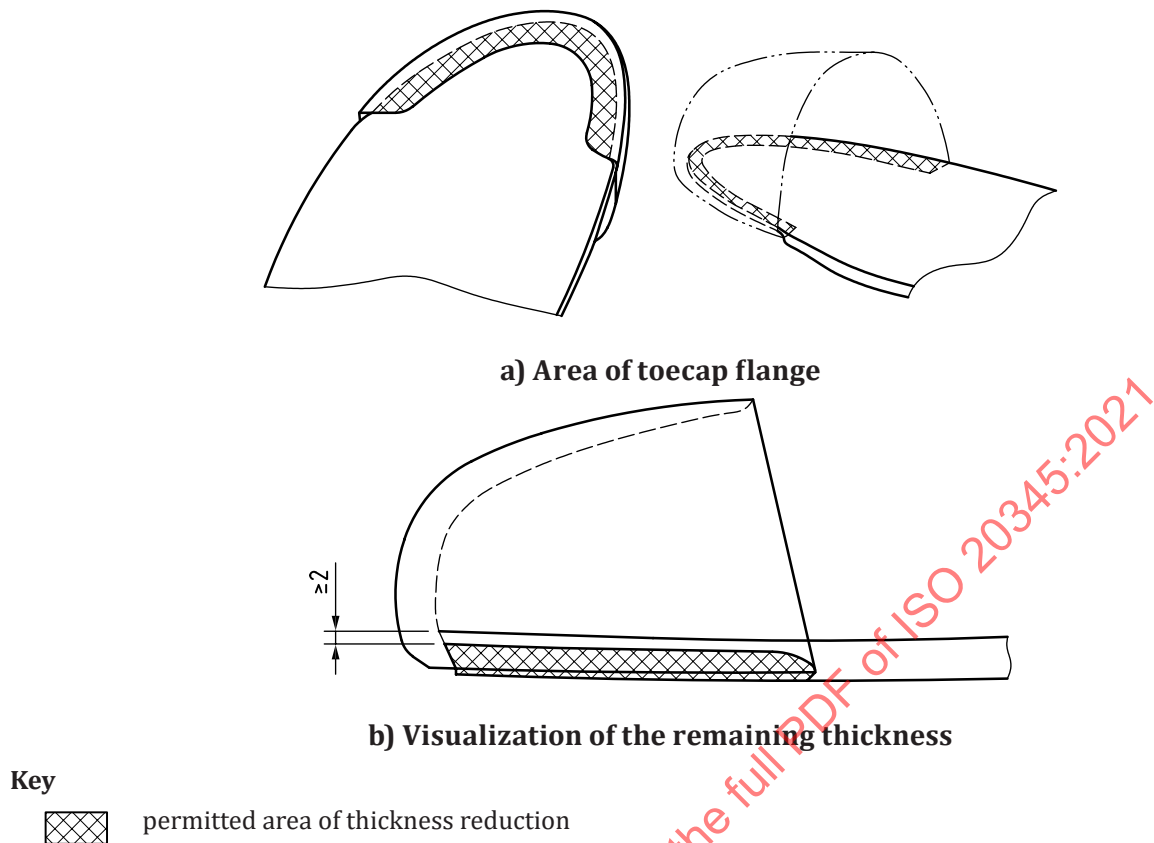
Figure 7 — Skiving area at toecap flange region
