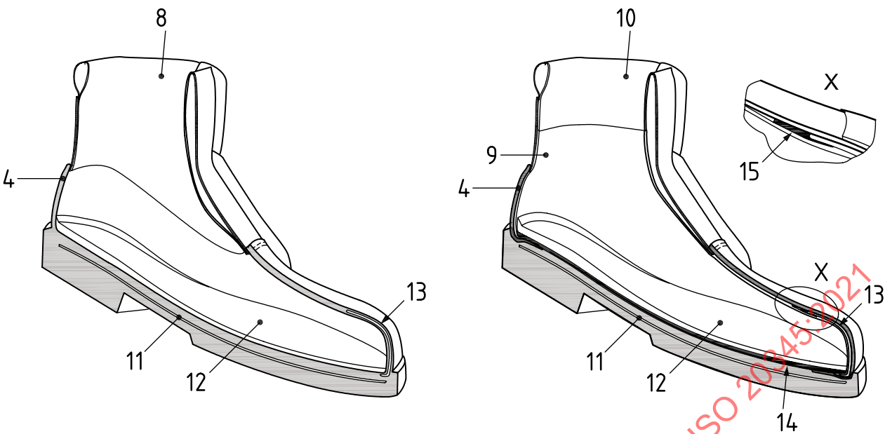
b) Hybrid moulded (entirely moulded lower section) c) Hybrid mounted (separately attached sole unit)
