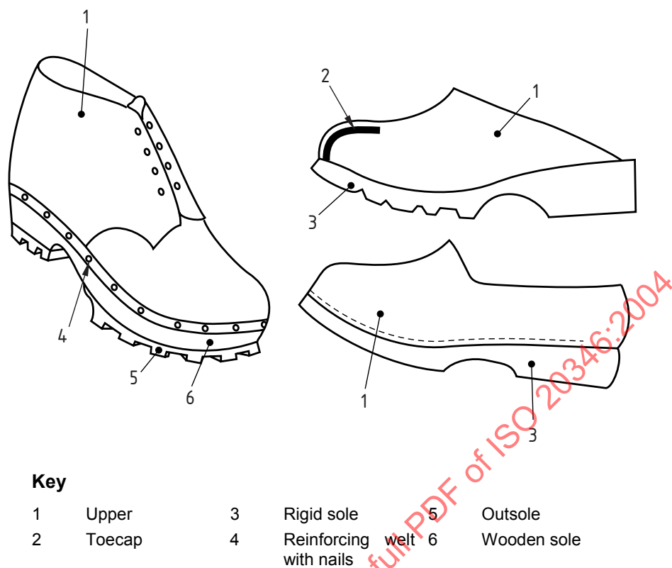
Figure 1b) Parts of footwear of conventional construction
