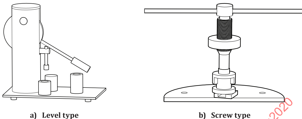
Figure 5 — Examples of a pellet presser
