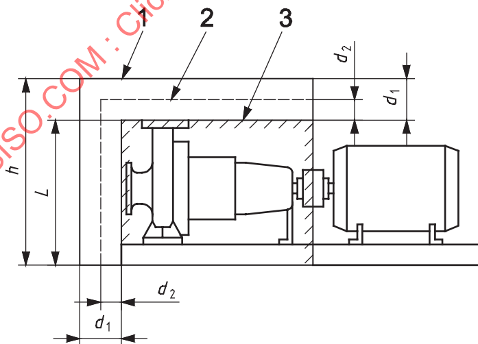
Figure 5 — Typical measurement surfaces and planes for sound intensity measurement for pump unit
