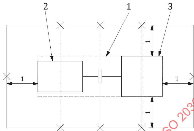
a) Median measurement surface
