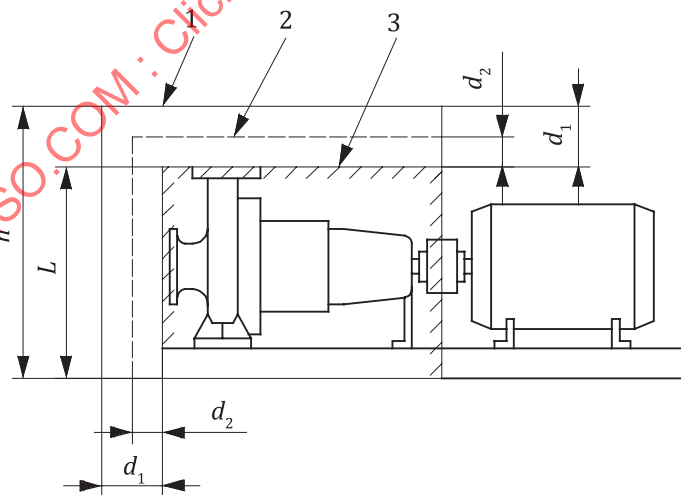
Figure 5 — Typical measurement surfaces and planes for sound intensity measurement for pump unit
