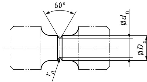
Figure C.3 — Schematic diagram of a notched test piece with a circular cross-section
