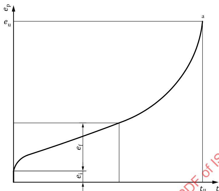
a) Extension-time diagram
