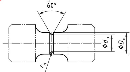
Figure C.3 — Schematic diagram of a notched test piece with a circular cross-section
