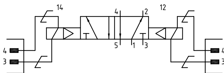
Figure 3 — Pin allocation for valves with double solenoids and two connectors
