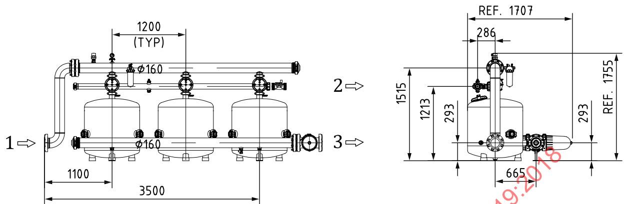
a) Gravel filtration batter
