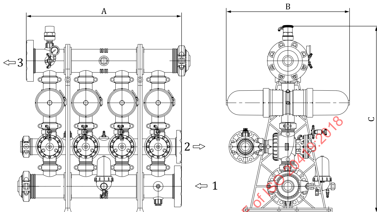
c) Disc filtration battery
