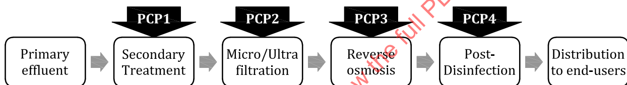
Figure 3 — Examples of PCPs in water reclamation plant for production of high quality reclaimed water
