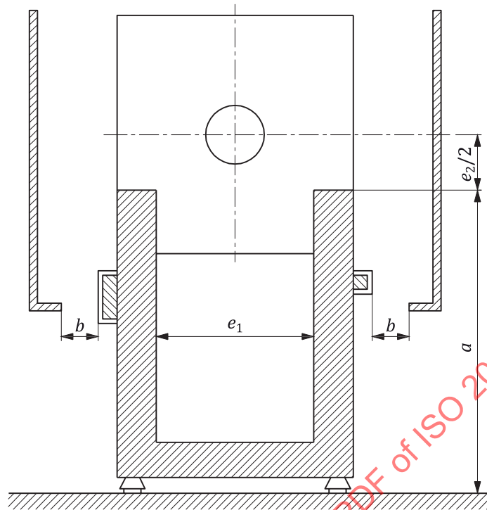
Figure 10 — Examples of the positioning of movable guards and dimensions a , b , e_1 , e_2 for machines with horizontal clamping unit without tie-bars
