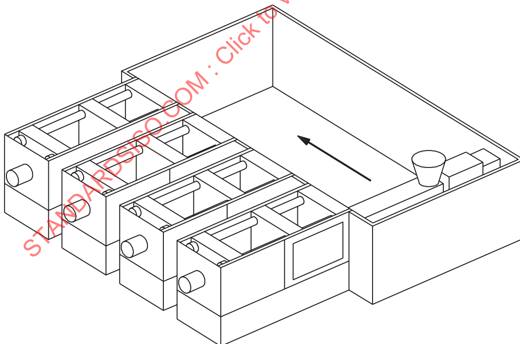
Figure 5 — Example of multi-station machine with mobile injection unit, shown with guards for the clamping units
