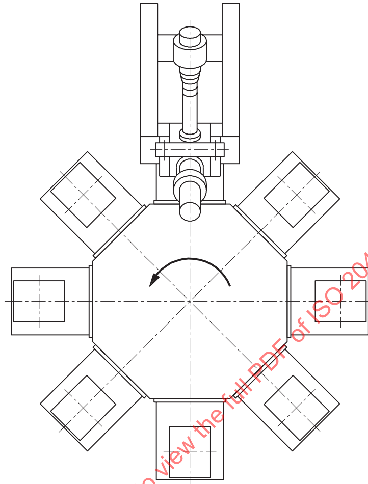
Figure 1 — Example of a carousel machine, shown without guards
