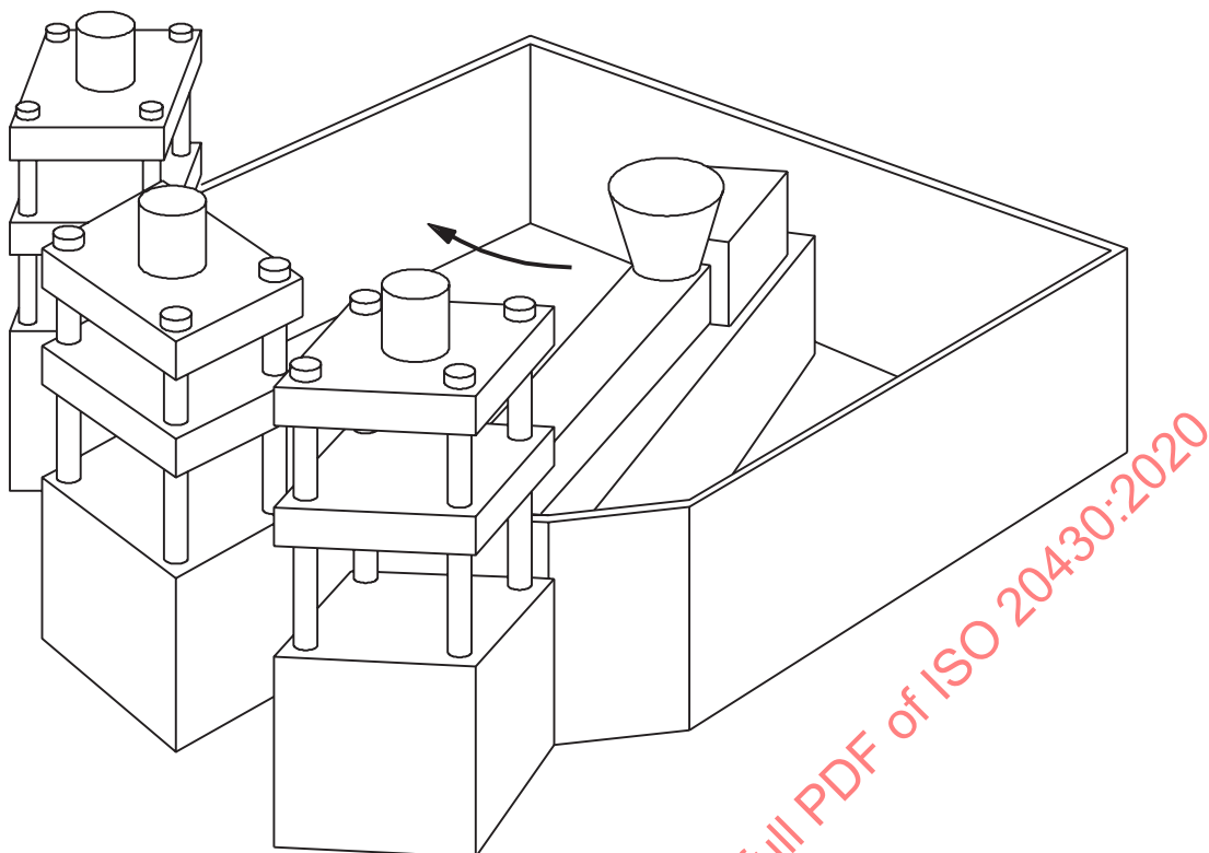
Figure 4 — Example of multi-station machine with mobile injection unit, shown without guards for the clamping units
