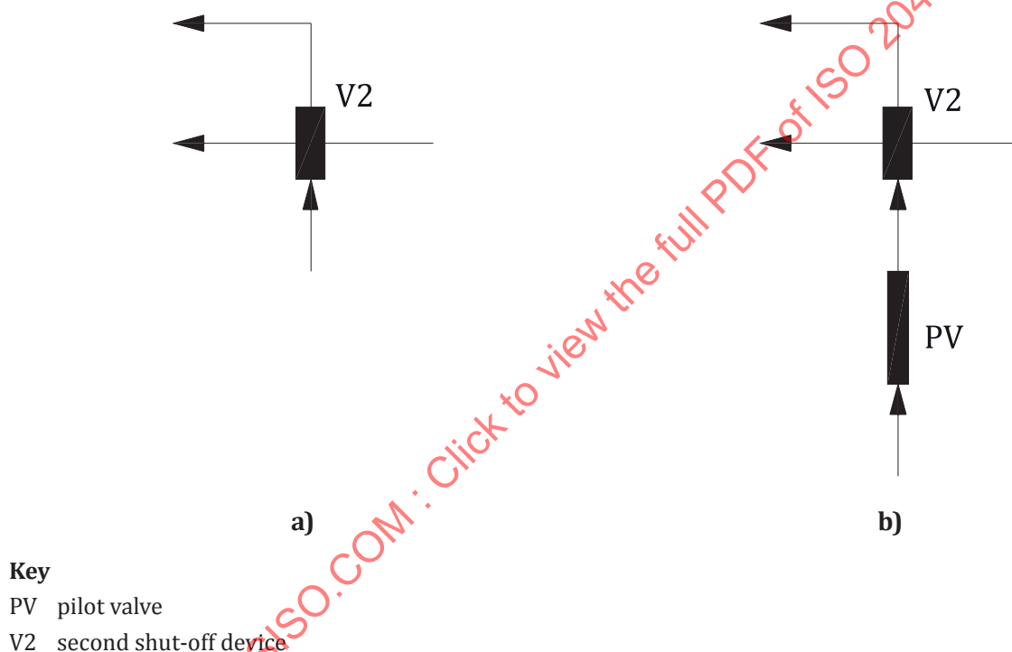
Figure D.17 — Alternatives for the actuation of the second shut-off device
