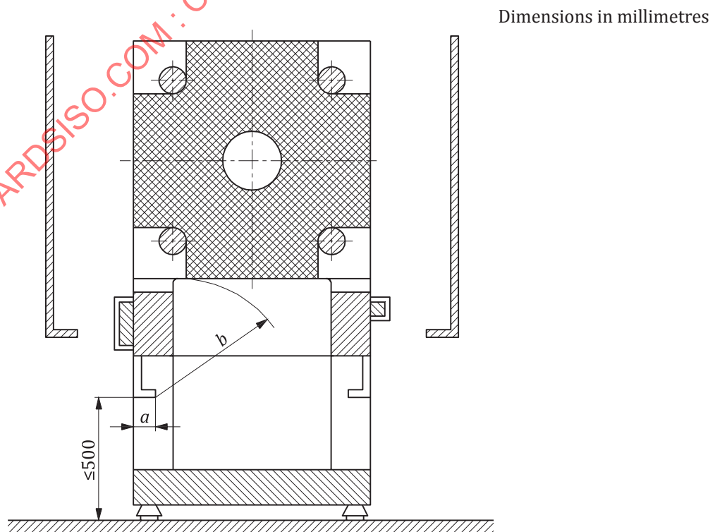
Figure 12 — Dimensions of the discharge area
