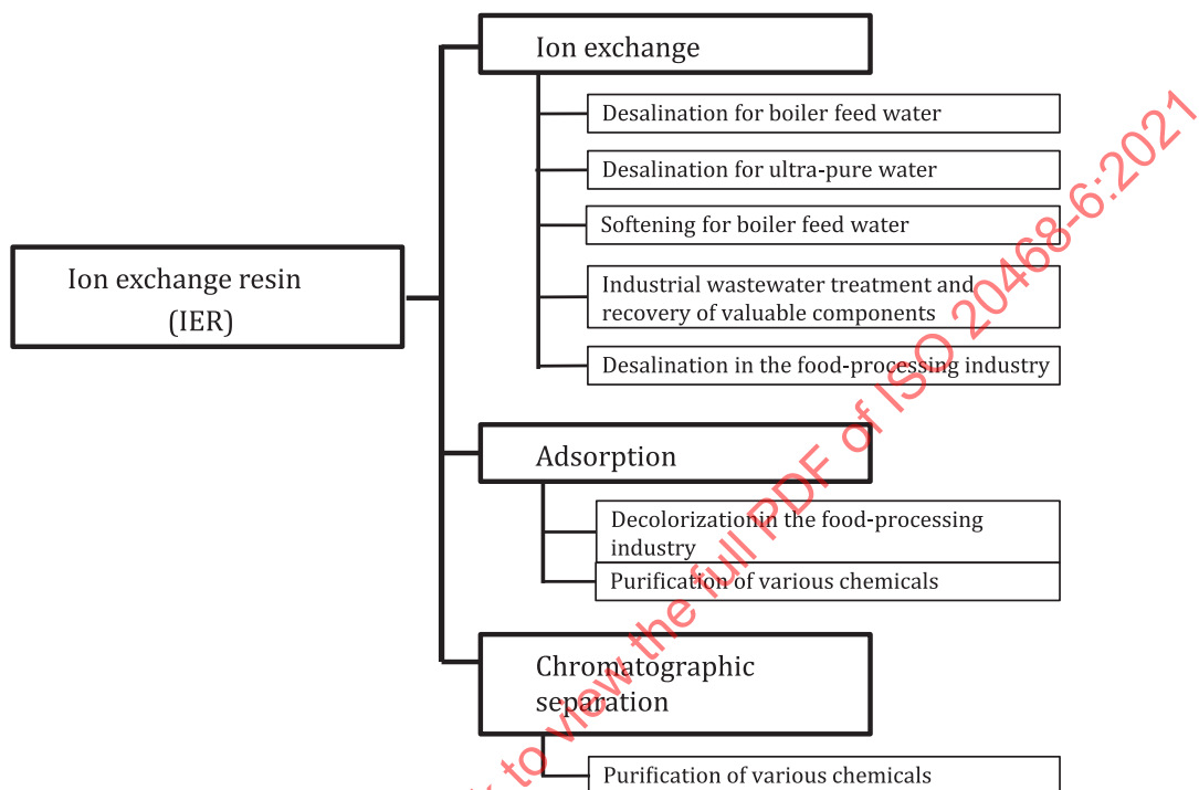
Figure A.1 — Main process and typical applications of IER
