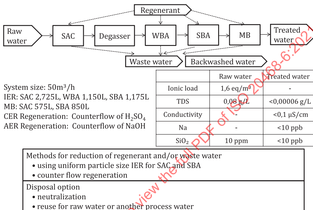
Figure G.1 — An examples of flow diagram and actual data of water treatment system by IER technology
