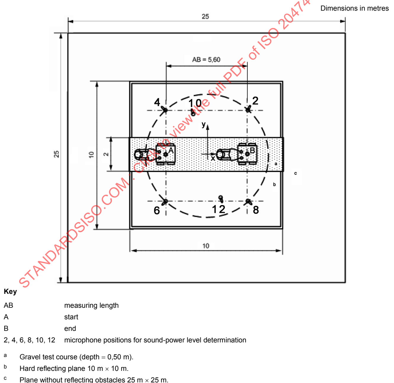
Figure A.1 — Test site and arrangement with test track
