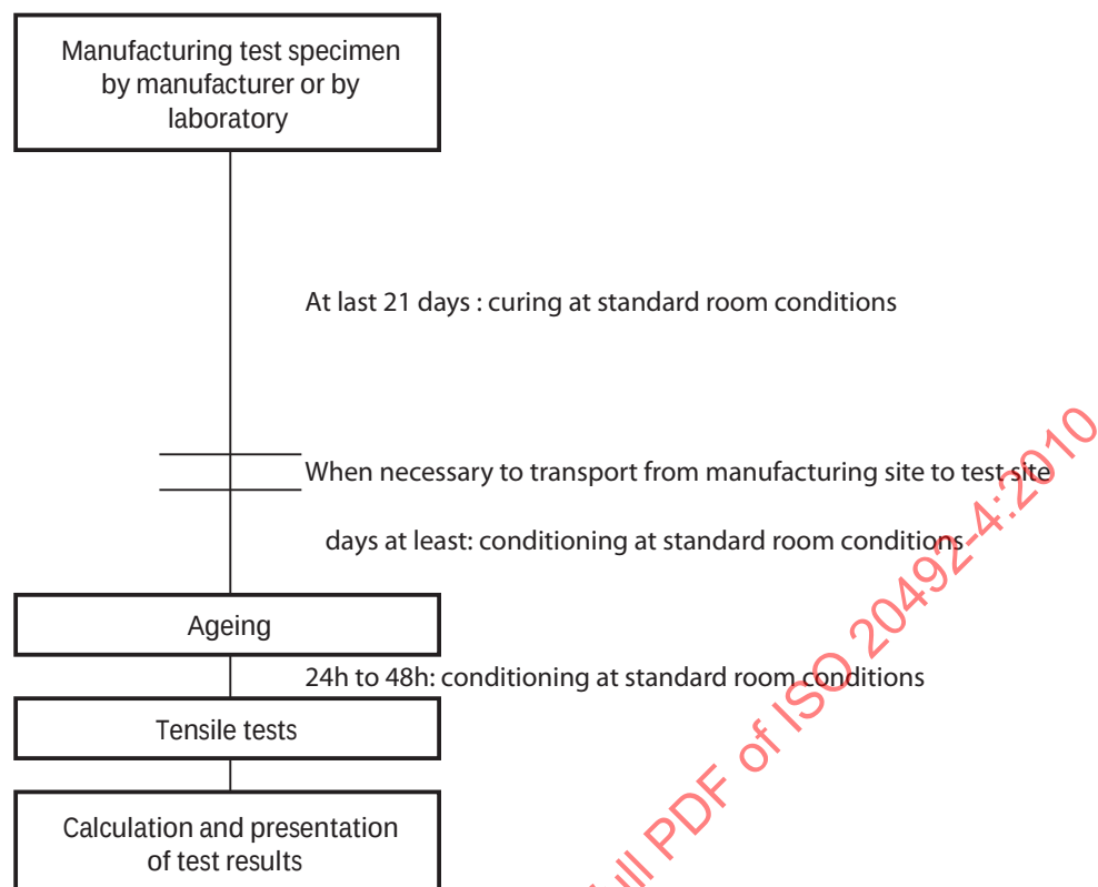
Figure 3 — Schematic presentation of test order for adhesion — Flow from top to bottom
