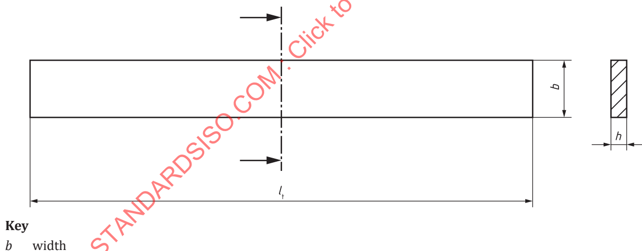
Figure 4 — Compression test specimen for use with grips (straight-sided, without tabs)
