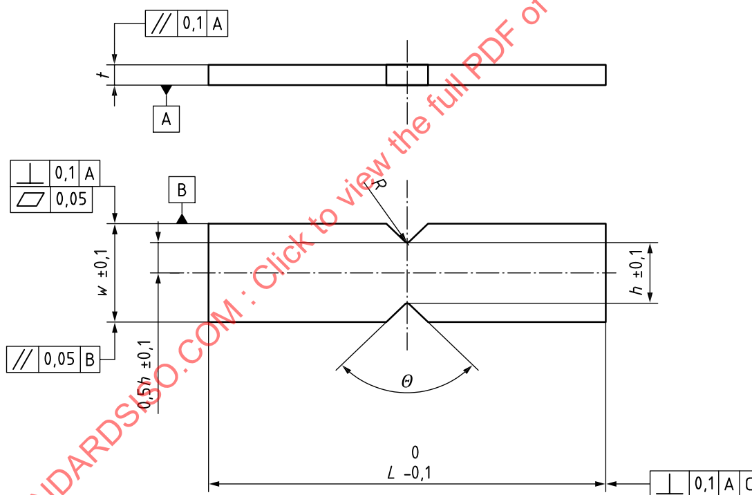
Figure 10 — Geometry and dimensions of Iosipescu test piece
