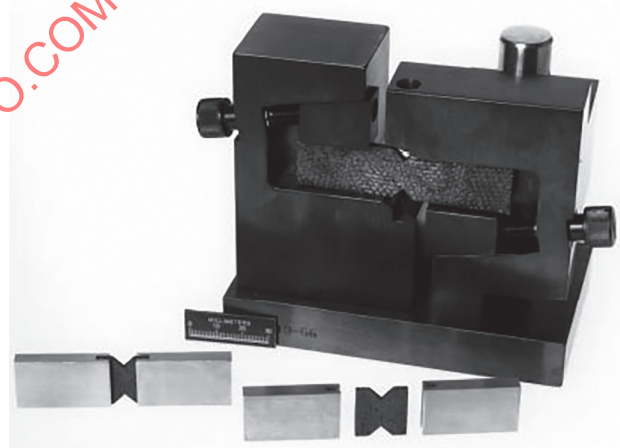
Figure 6 — Commercially available fixture for Iosipescu test
