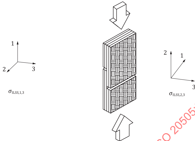
Figure 2 — Schematic of double-notched test piece subjected to compressive loading
