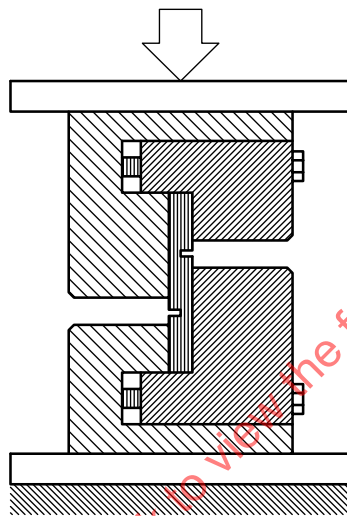
Figure 4 — Example of anti-buckling fixture for compression of double-notched test piece
