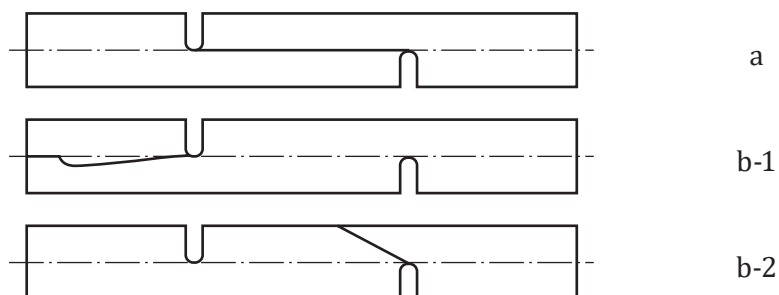
Figure 12 — Examples of valid and invalid ruptures for the Iosipescu test
