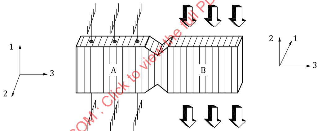
Figure 3 — Schematic of Iosipescu test piece
