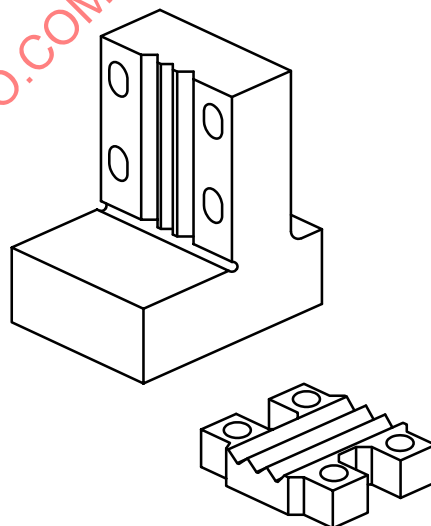
Figure 5 — Example of anti-buckling fixture for compression of double-notched test piece
