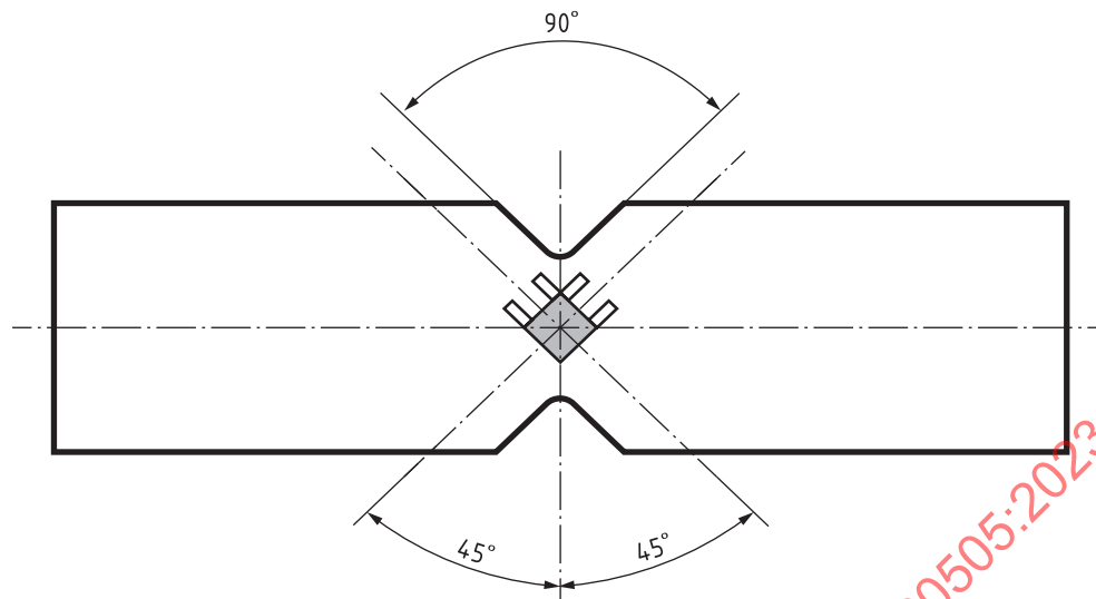
Figure 8 — Example of test specimen equipped with strain gauges: superposed strain gauges, bonded in the centre and at 45° from the axis
