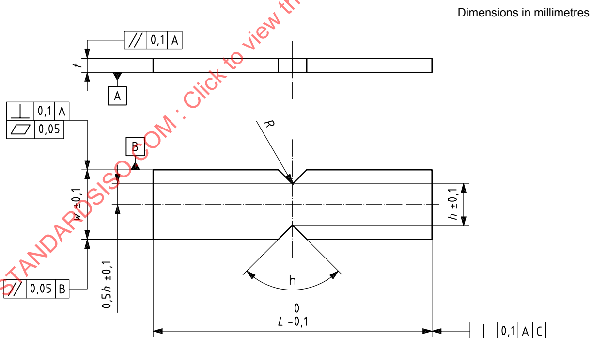
Figure 2 — Geometry and dimensions of Iosipescu test piece
