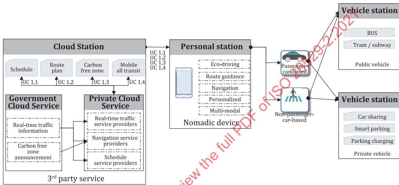
Figure 2 — Route selection service flow
