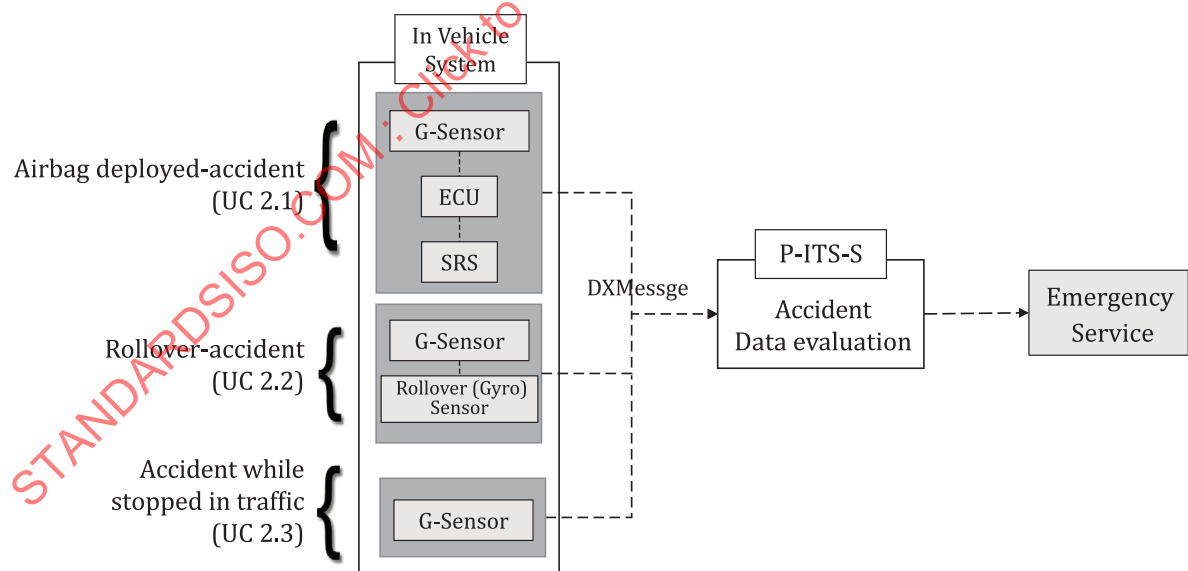
Figure 1 — Accident detection reference system
