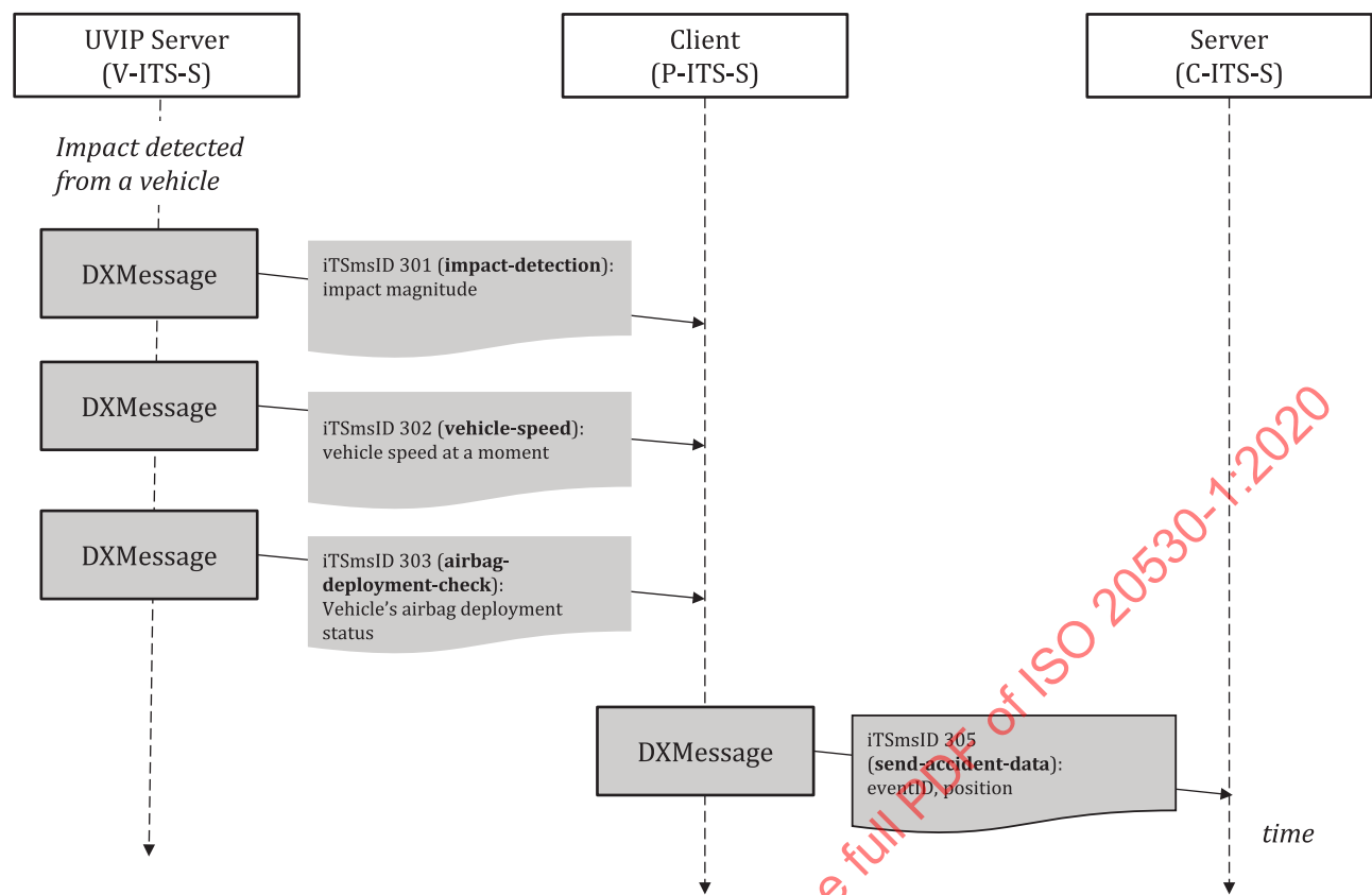
Figure 2 — Message flow of impact detection
