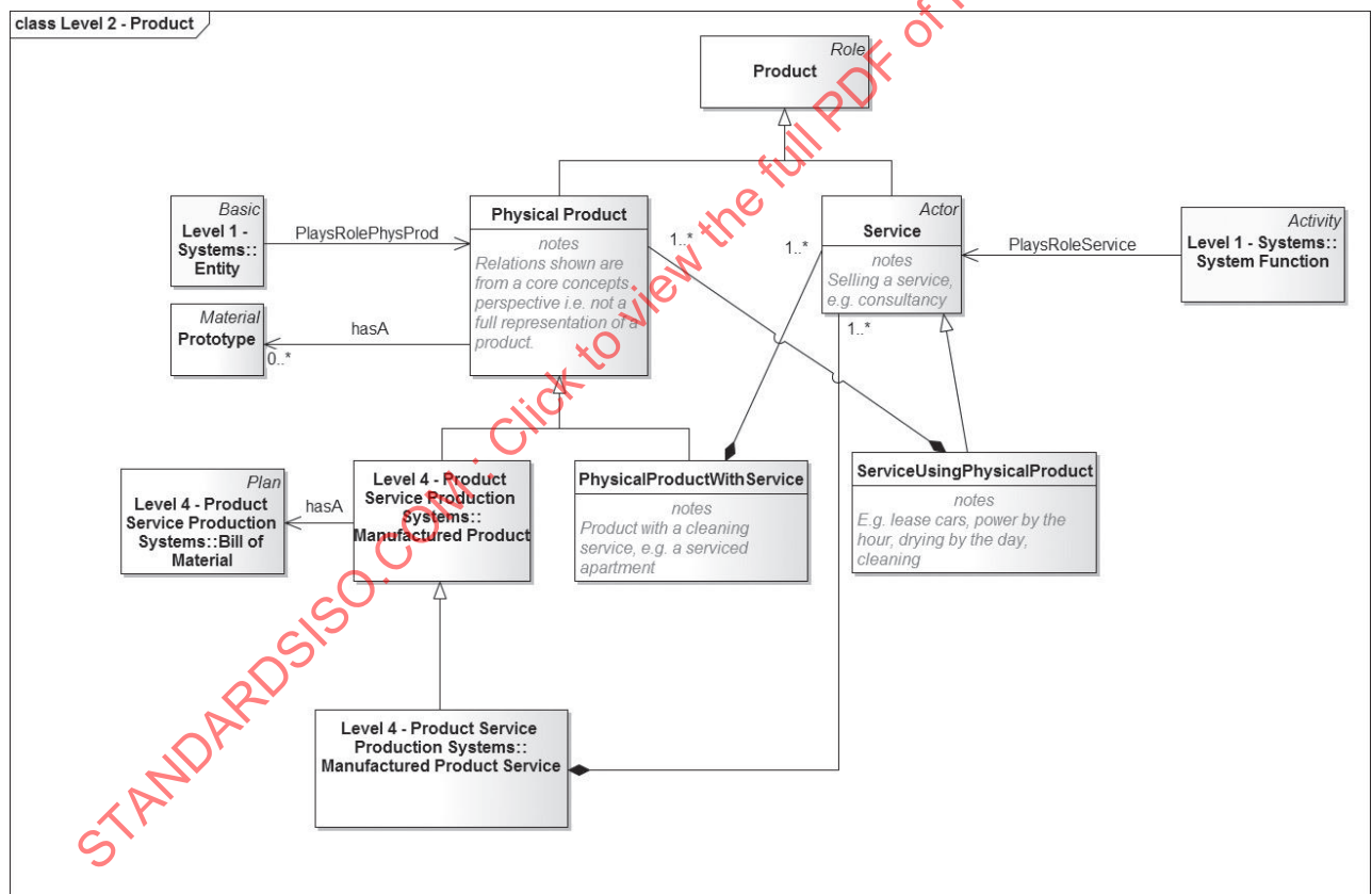
Figure 7 — UML class diagram depicting the representation of product at levels 2 and 4
