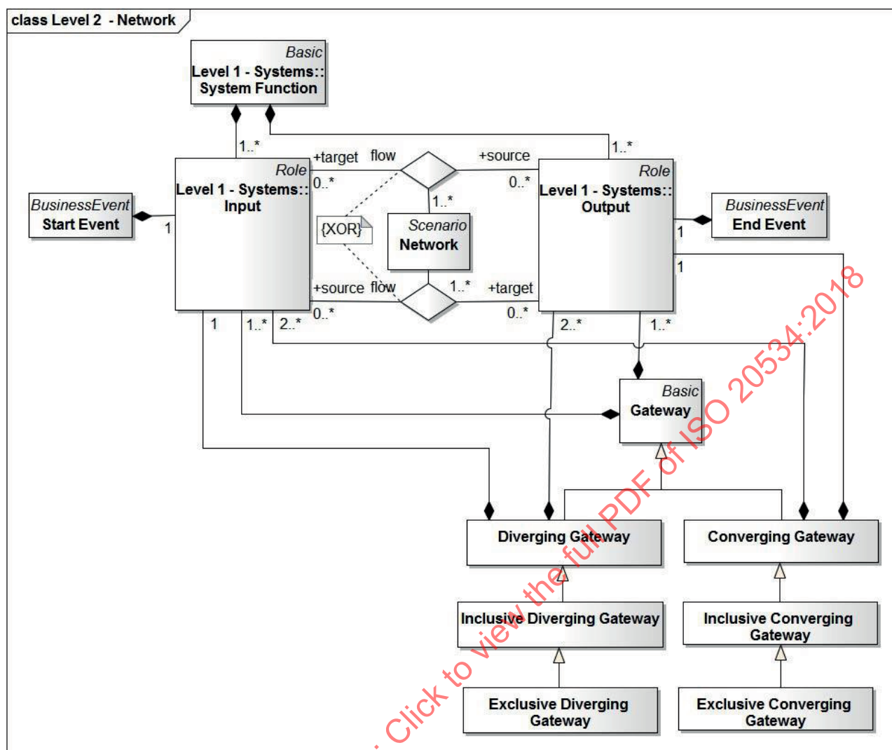
Figure 6 — UML class diagram depicting the representation of network at level 2
