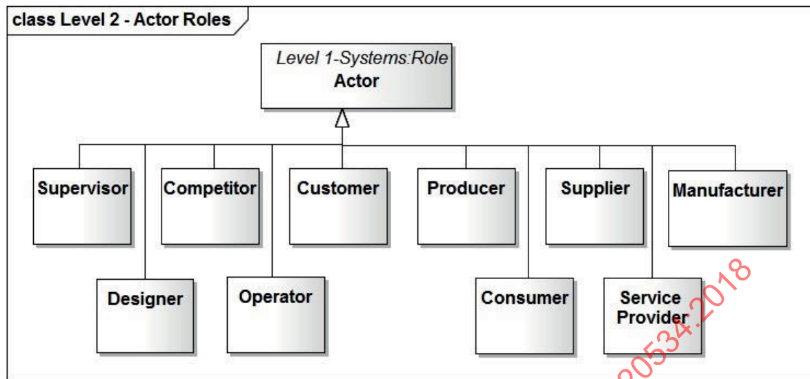
Figure 5 — UML class diagram depicting roles, especially actor roles
