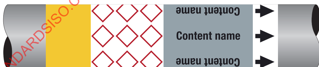
Figure C.11 — Example of a pipe marker with a hazardous content according to an SDS, the GHS pictograms on a white background and the flow direction indicator in black on a white background
