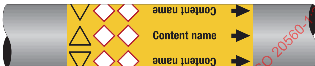
Figure C.13 — Example of a pipe marker with a hazardous content according to an SDS and risk assessment, the content name, warning sign, GHS pictograms and the flow direction indicator placed in the yellow safety colour
