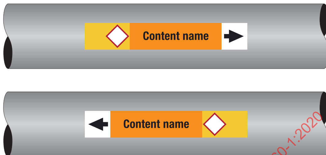
Figure C.15 — Examples of a single pipe marker with a hazardous content according to an SDS, a GHS pictogram on the yellow safety identification colour and the flow direction indicator in black on a white background
