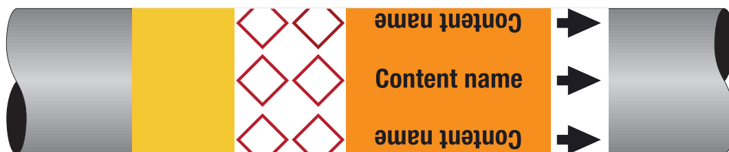
Figure C.4 — Example of a pipe marker with a hazardous content according to an SDS, GHS pictograms on a white background and the flow direction indicator in black on a white background
