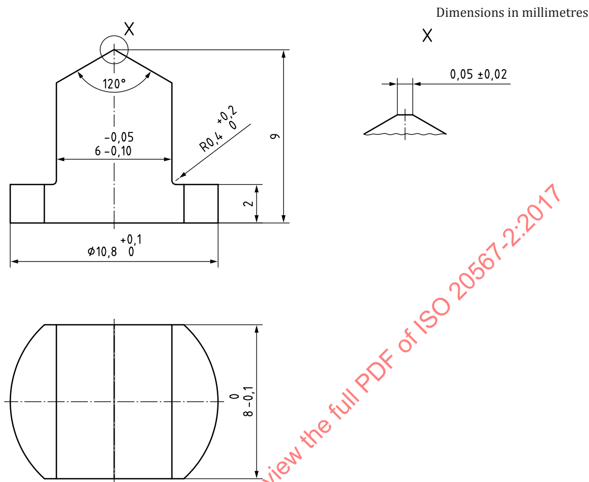
Figure 2 — Impact body
