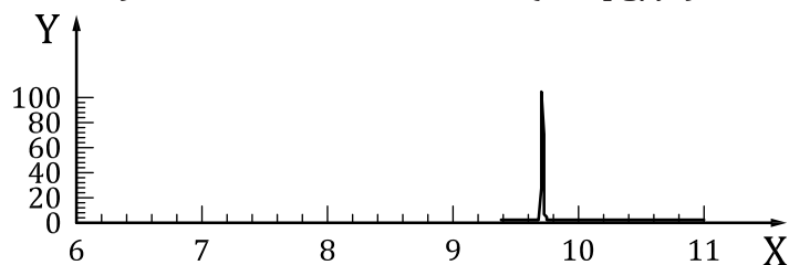
e) Extracted ion for D6 (100 pg/μl)
