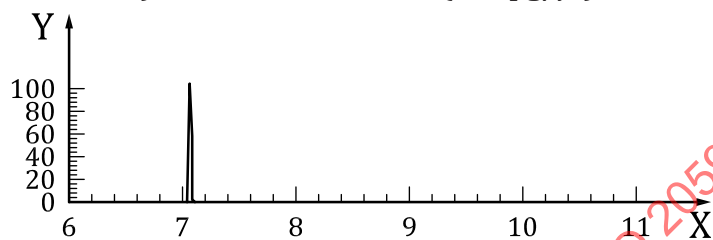
b) Extracted ion for ^{13}\text{C}_4\text{-D4} (100 pg/μl)
