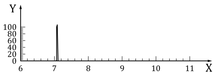
a) Extracted ion for D4 (100 pg/μl)
