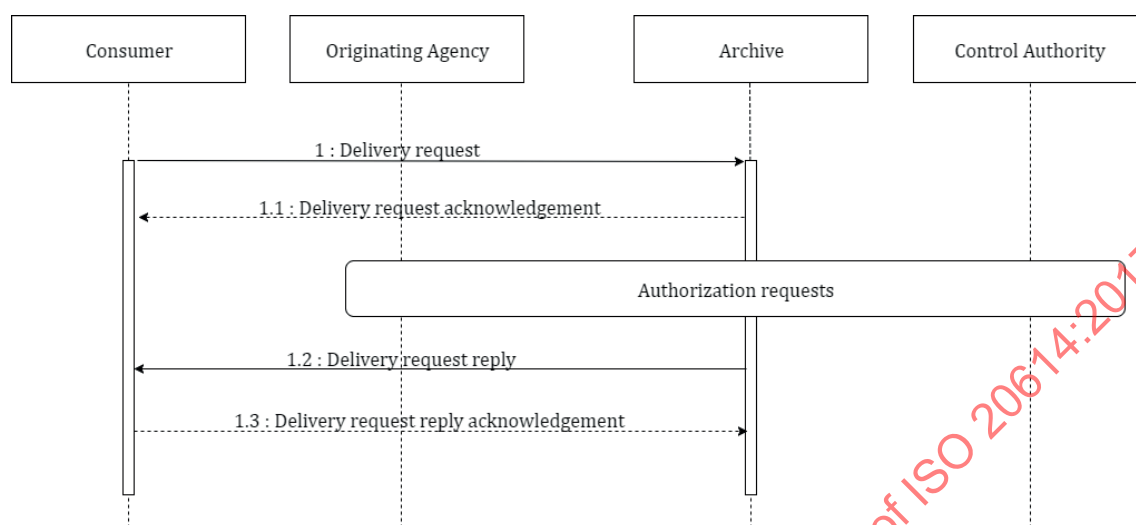
Figure 8 — Sequence diagram: Deliver
