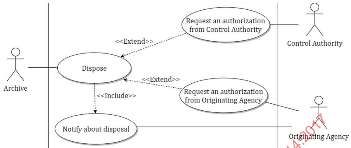
Figure 5 — Use case diagram: Dispose
