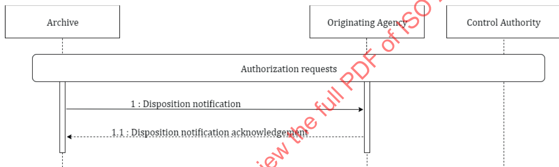
Figure 10 — Sequence diagram: Dispose
