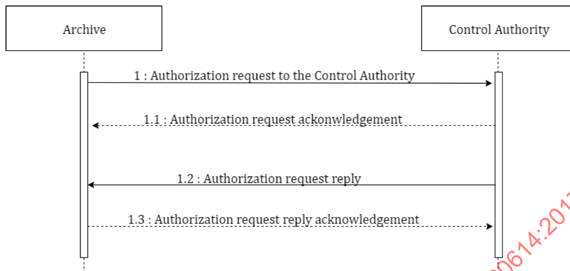
Figure 13 — Authorization request to the Control Authority
