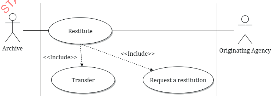
Figure 6 — Use case diagram: Restitute
