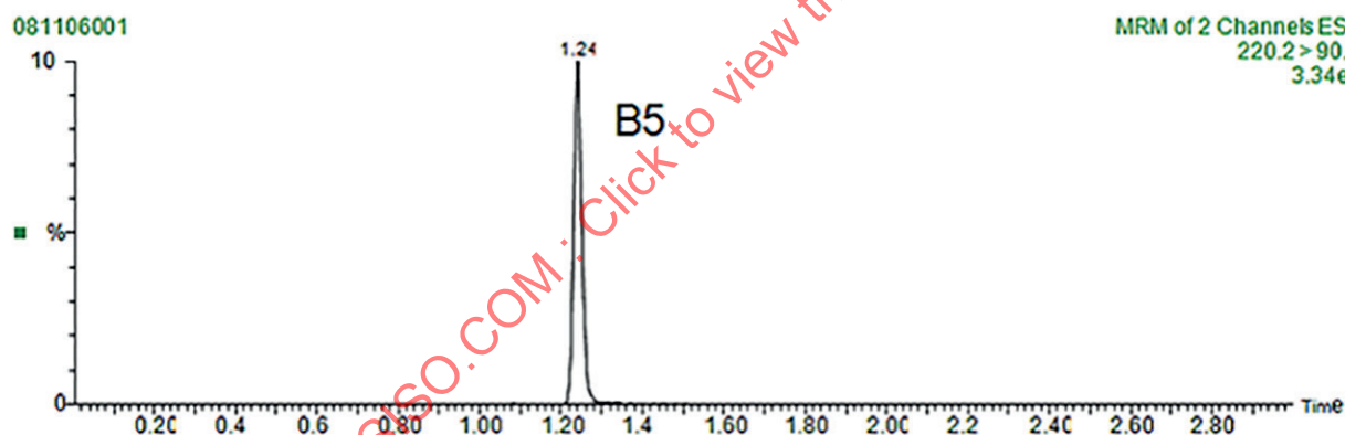
Figure A.2 — Chromatogram of pantothenic acid in an infant formula sample by UHPLC-MS/MS
