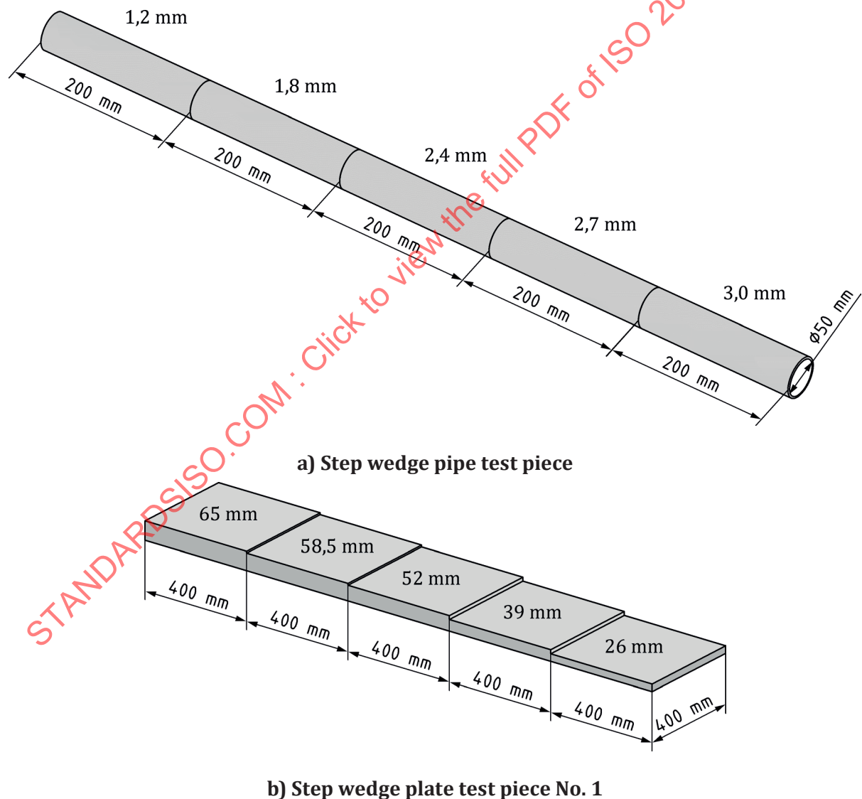
Figure 3 — Reference blocks
