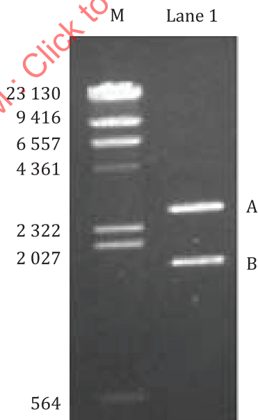
Figure C.2 — Restriction digestion analysis of synthetic gene of 246 bp in 3,1 kb vector (1 % agarose gel)
