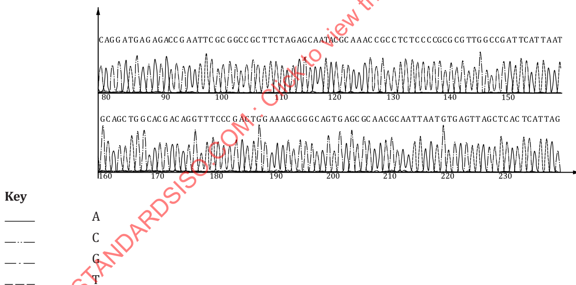
Figure D.1 — Verification of a GFY gene by Sanger sequencing
