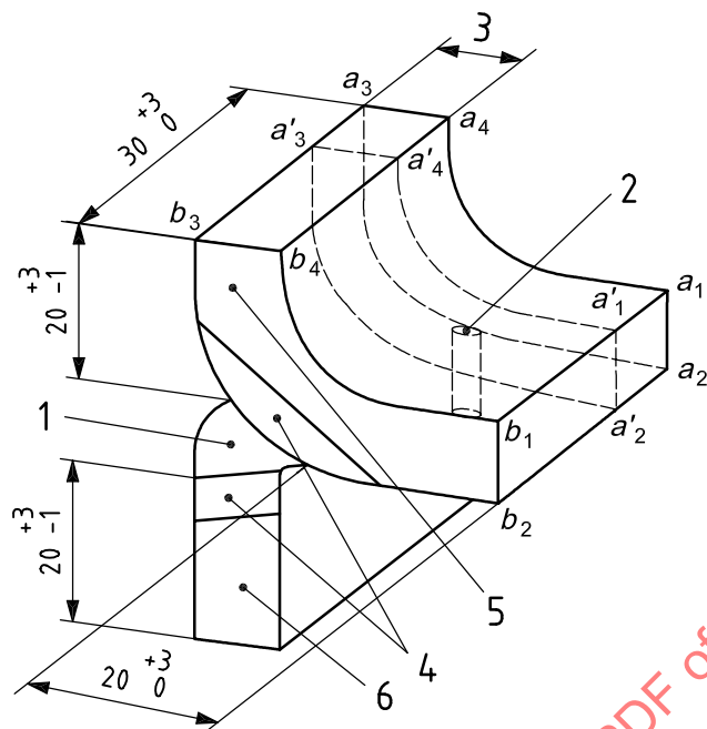
b) Details of WC2 test piece
