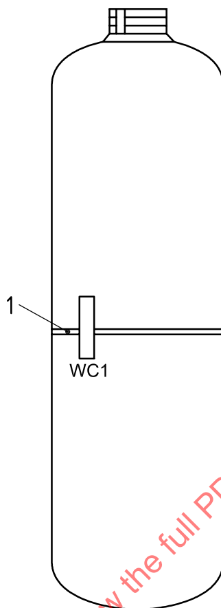
a) Cylinders with circumferential seams only
