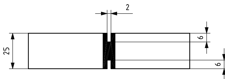
Figure 6 — Nick-break test on weld
