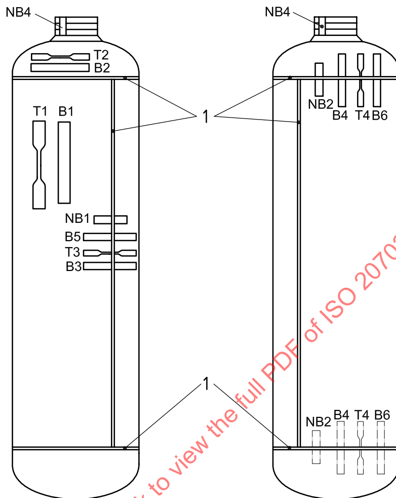
d) Cylinders with longitudinal and circumferential seams
