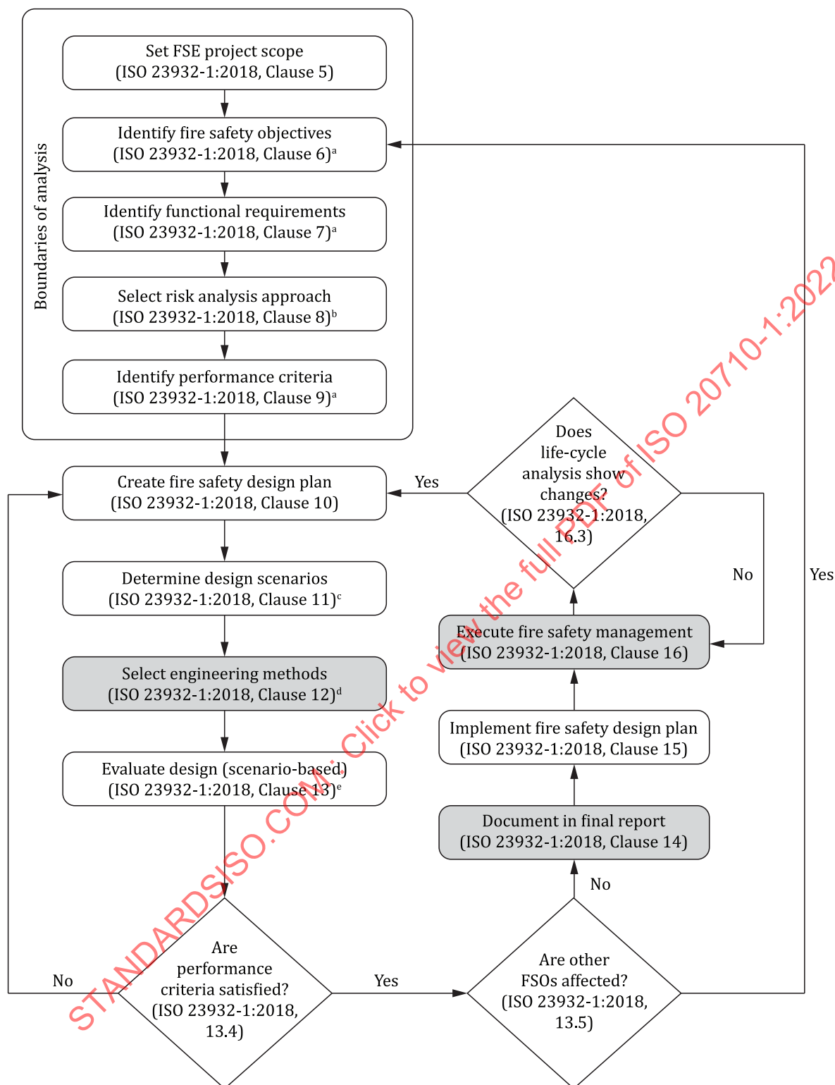
Figure 1 — Flow chart illustrating the fire safety engineering design process (from ISO 23932-1:2018)
