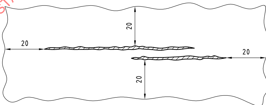
Figure 3 — Determination of the area affected by aligned single or multiple discontinuities
