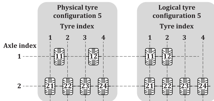
Figure B.10 — Tyre pressure - Vehicle with dual tyres on rear axle example
