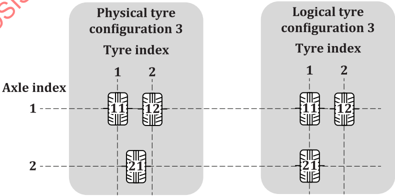
Figure B.8 — Tyre pressure - Trike reverse example
