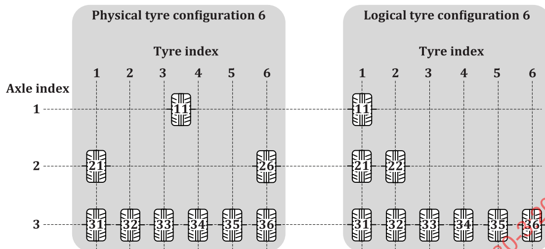
Figure B.11 — Tyre pressure - Vehicle with >6 tyres configuration 1 example
