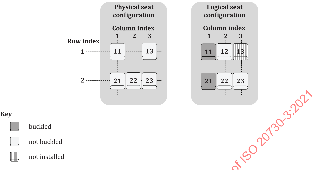
Figure B.2 — Seat belt buckle – 5-seater single ECU example
