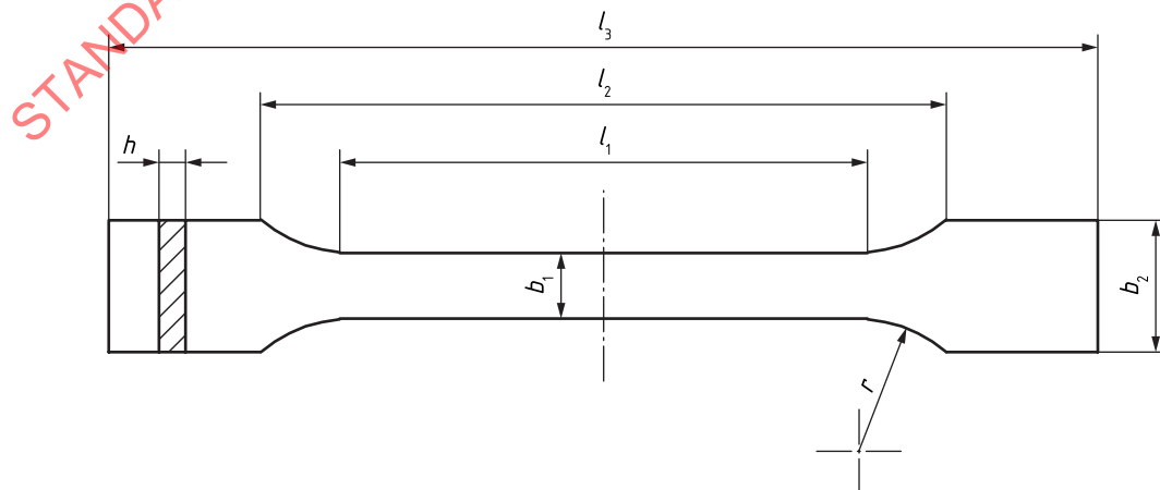
Figure 1 — General design of tensile test specimens
